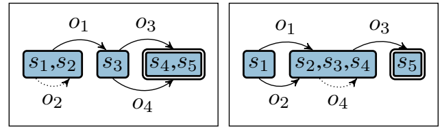
Figure 1: Example abstraction heuristics (Figure 1 in Seipp, Keller, and Helmert 2017a). The cost function is cost = \{o_1 \mapsto 4, o_2 \mapsto 1, o_3 \mapsto 4, o_4 \mapsto 1\} . The s_i are concrete states, the rounded rectangles are abstract states, abstract goal states use double borders and dotted lines depict abstract self-loops.
